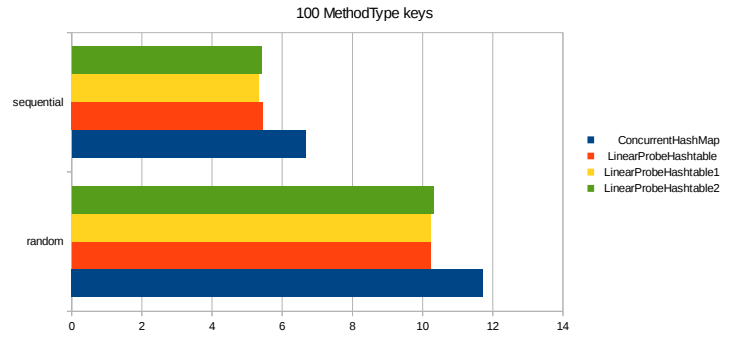
MethodType lookup
