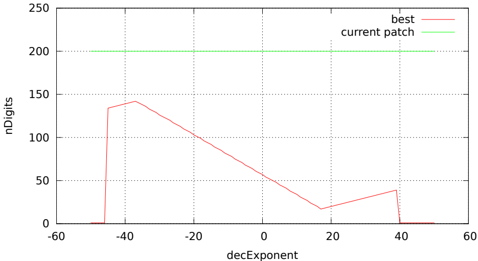
Sufficient nDigit as function of decExponent for Float format
