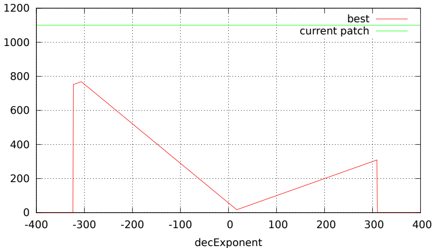
Sufficient nDigit as function of decExponent for Double format
